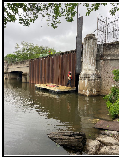
Figure 2: Driscoll Construction completing cofferdam work.
