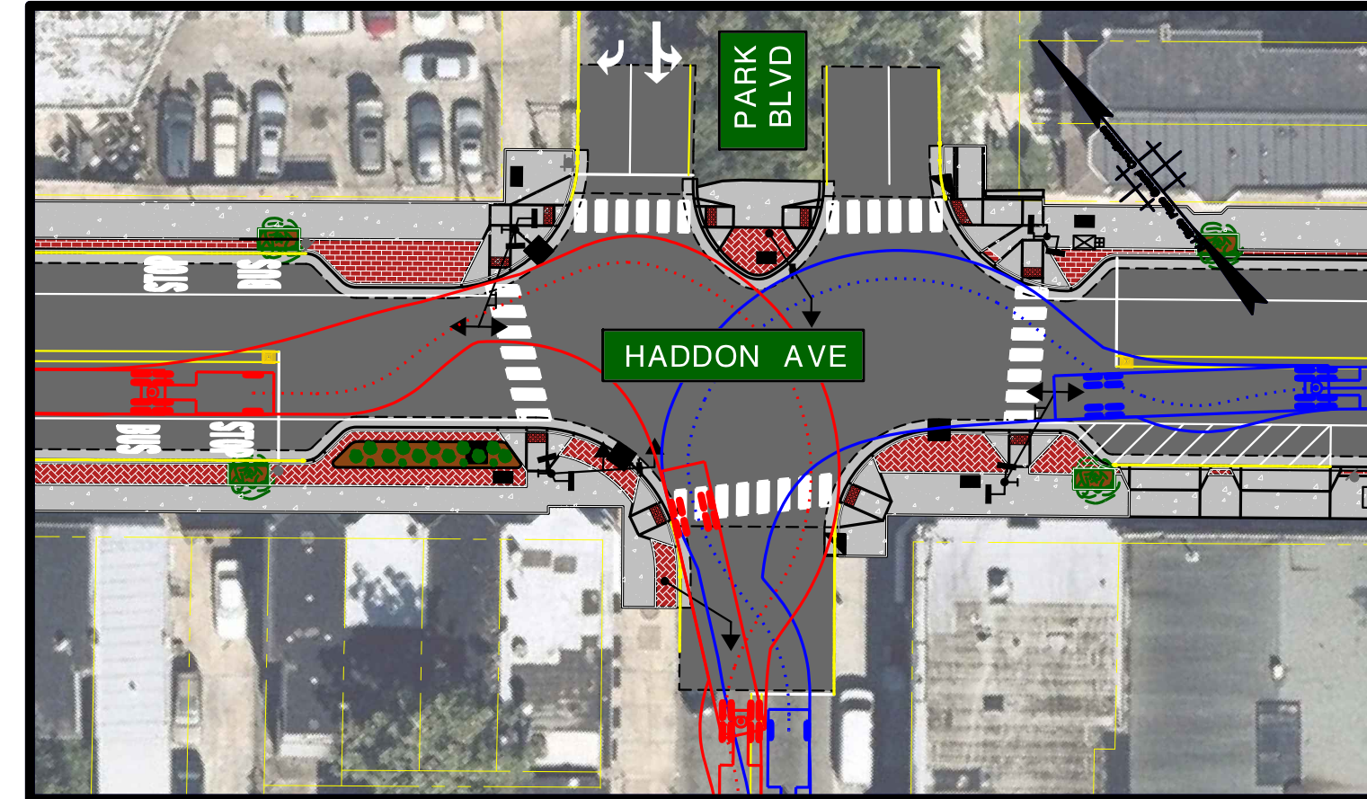
WB-62 TURNS AT PARK BOULEVARD
