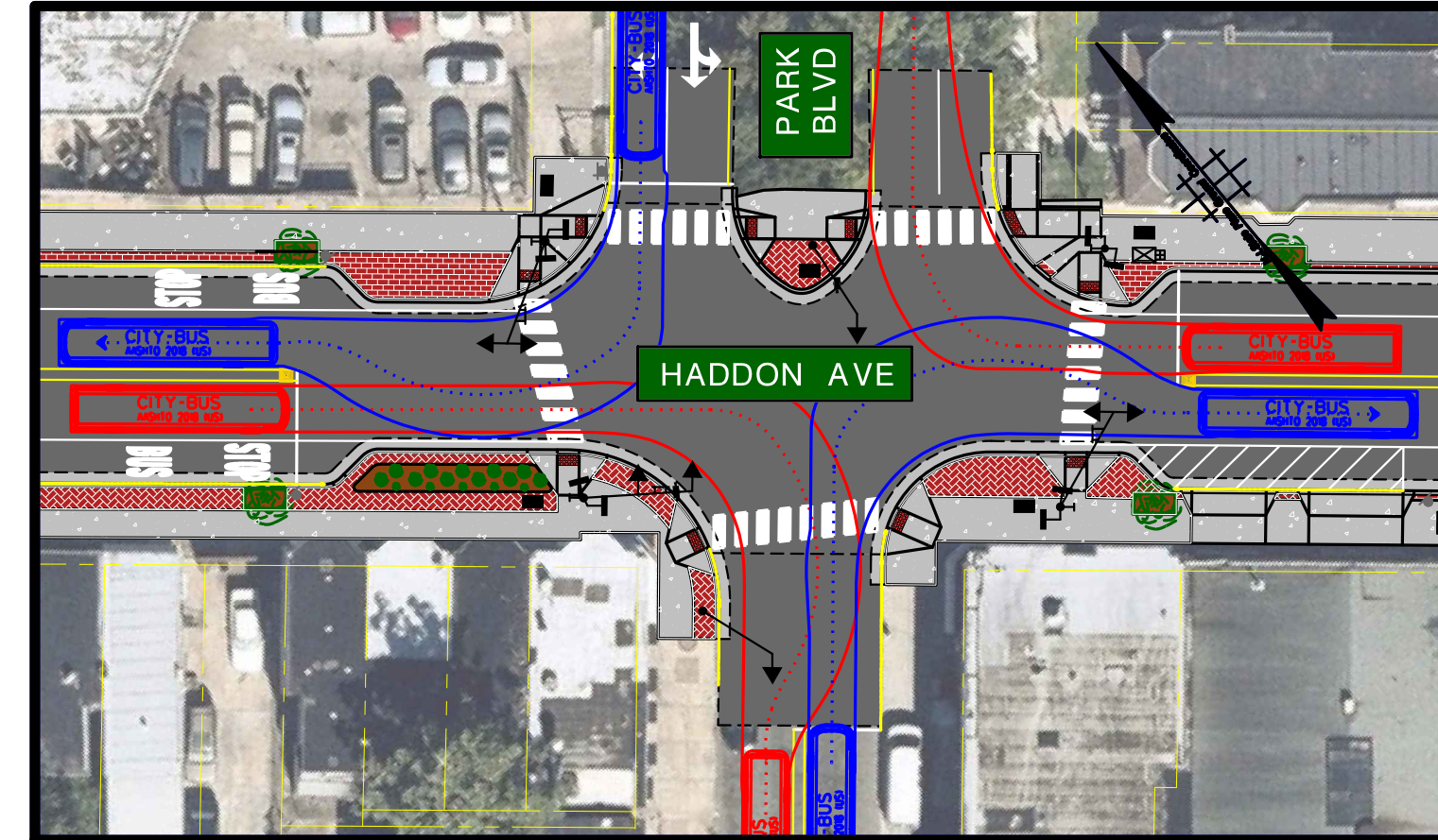
BUS TURNS AT PARK BOULEVARD
