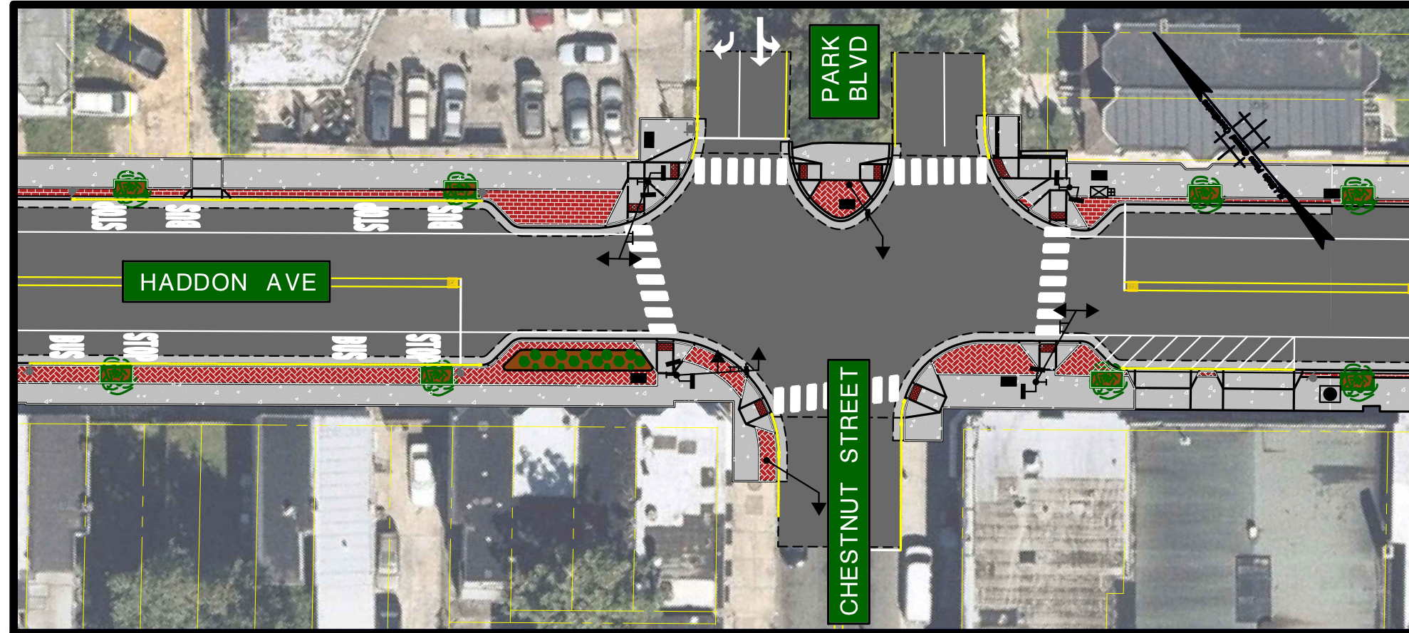
HADDON AVE & PARK BOULEVARD INTERSECTION
