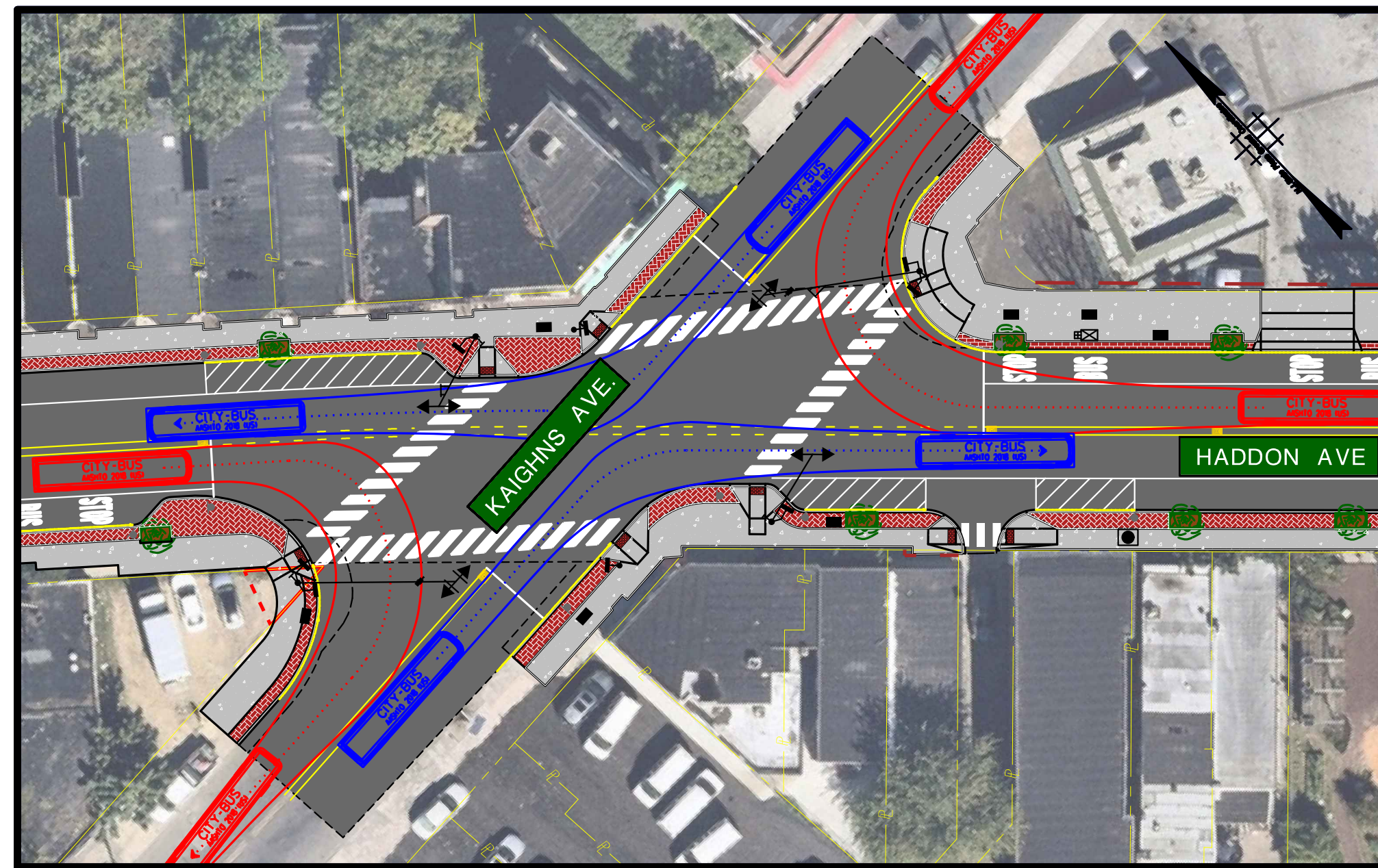
BUS TURNS AT KAIGHNS AVENUE
