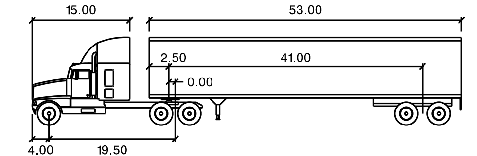
WB-62 Modified (WB-67 Trailer with modification) Tractor Width : 8.00 Trailer Width : 8.50
