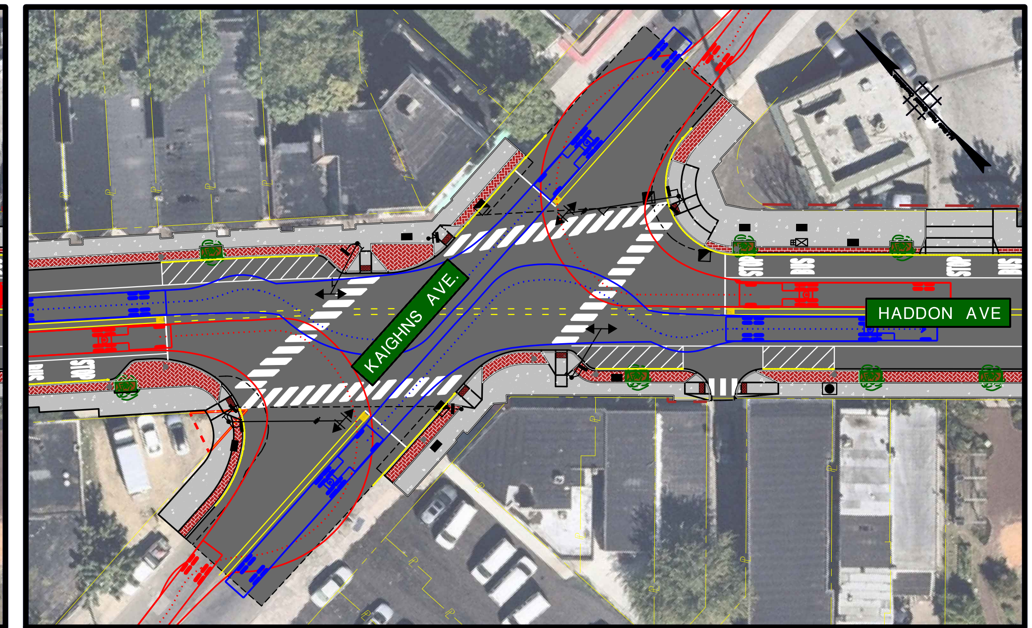
WB-62 TURNS AT KAIGHNS AVENUE
