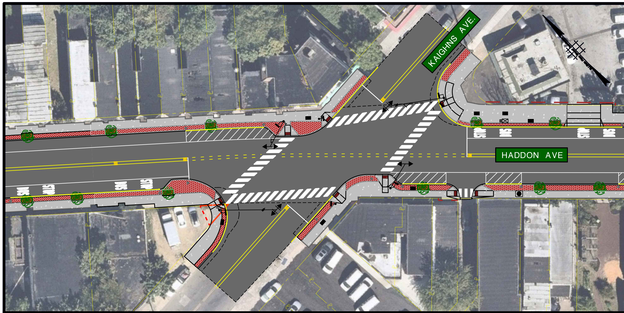
HADDON AVE & KAIGHNS AVENUE INTERSECTION
