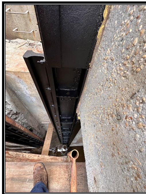
Figure 3: New Crane Rails.
