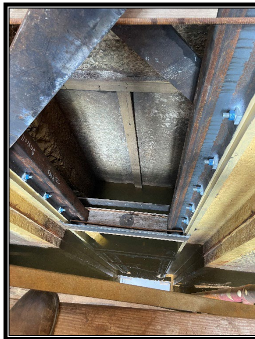
Figure 3: New Crane Rails set East side.
