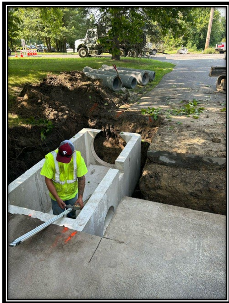
Figure: 1 – Installation of Type Double B Inlet and 12” RCP at the intersection with Hamilton Street
