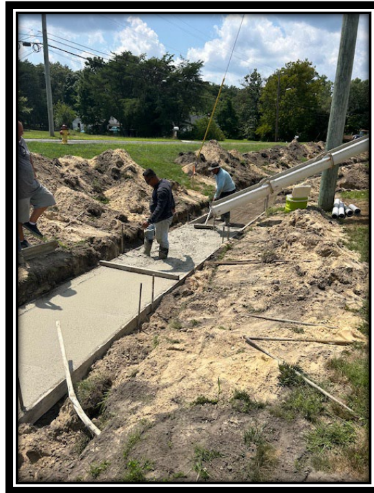
Figure: 2 – Installation of 6" thick, reinforced concrete drainage swale along the frontage of 117 Jackson Road
