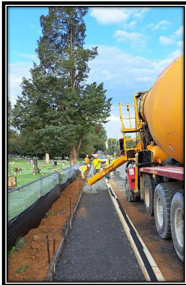
Figure: 1 – Installation of concrete sidewalk along the eastbound lane between Millstream Drive and King’s Highway
