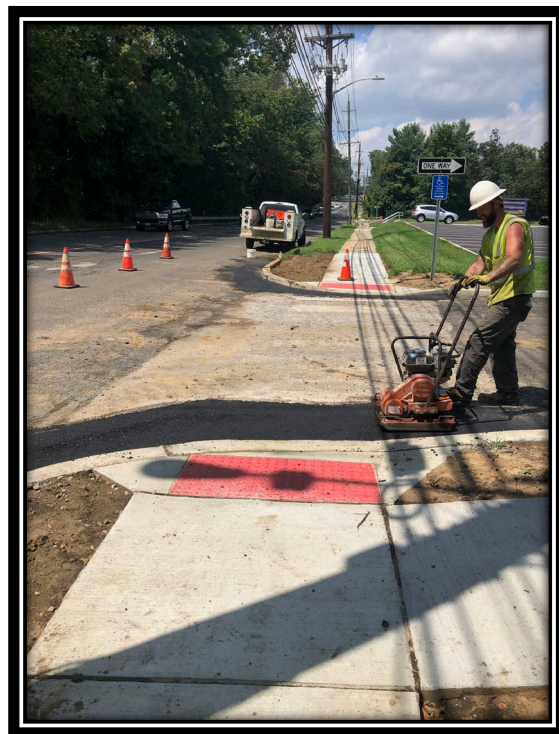
Figure: 3 – HMA restoration around newly installed ADA ramp and curb along the westbound lane in front of the Thomas Paine Elementary School
