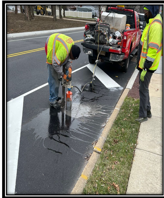
Figure: 3 – Coring of newly installed HMA surface and base course as per NJDOT materials testing requirements along the westbound lane between King’s Highway and Millstream Drive
